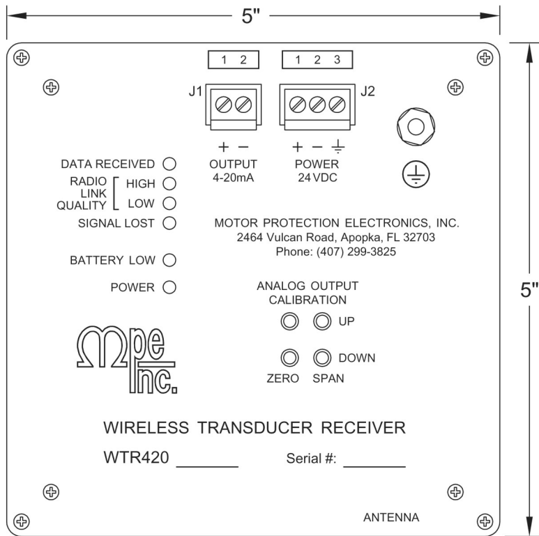
Receiver Front
