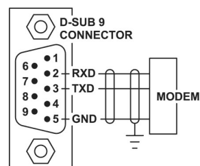
RS-232 Serial Port
